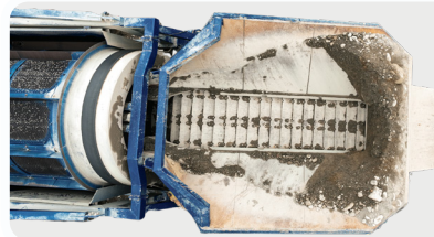
APRON FEEDERS
