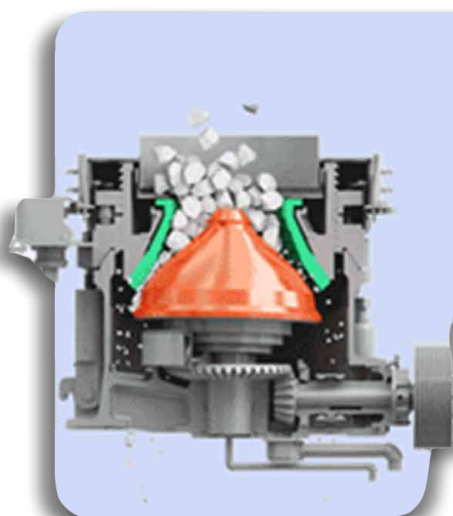
CONE CRUSHER
